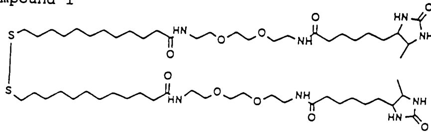
desthio compound 1
